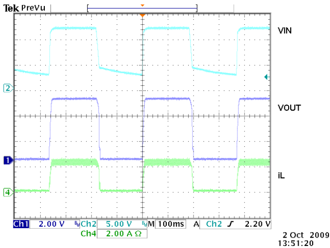
Figure 9. Input power recycling
