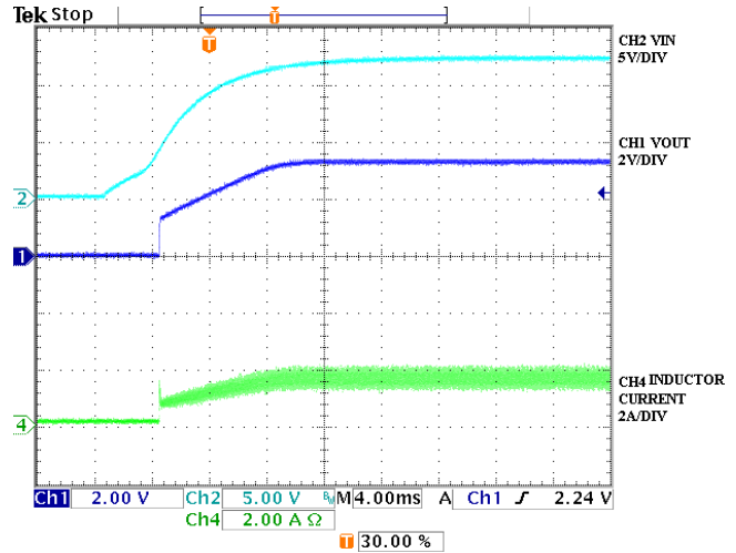
Figure 8. Start up with 1.5A load
