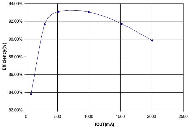
Figure 9. Efficiency vs. IOU(VIN=12V,VOUT=5V)
