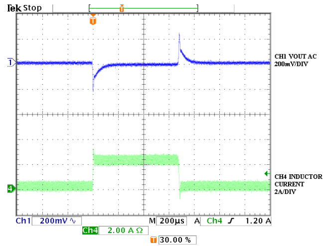
Figure 6. Transient Response
