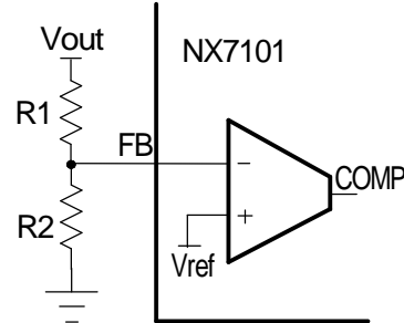
Figure 5 Voltage Divider
