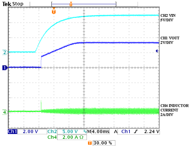
Figure 7. Start up with no load
