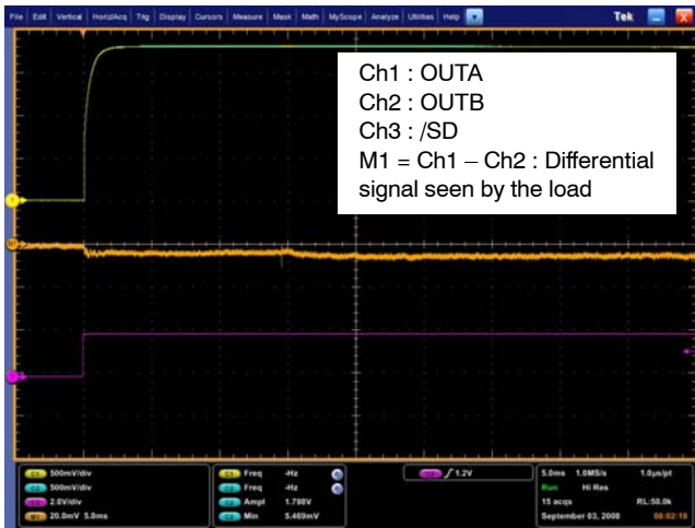
Figure 33. Zero pop noise turn on sequence with single-ended input to ground ( C_i = 47 \text{ nF} , R_i = 24 \text{ k}\Omega , R_f = 24 \text{ k}\Omega , C_{byp} = 1 \text{ }\mu\text{F} , R_l = 8 \text{ }\Omega , T_{on} = V_p )
